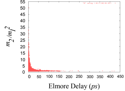
Figure 7: The distribution of m_2/m_1^2 for RC trees and ladders in the 90nm design testcase.
