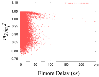
Figure 6: The distribution of m_2/m_1^2 for RC ladder interconnects in the 90nm design testcase.
