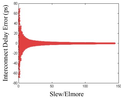
Figure 12: Interconnect delay error versus slew over Elmore delay for the 90nm design testcase.
