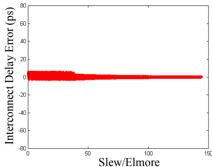
Figure 14: The calculated delay of the 90nm design testcase based on filtering algorithm with \phi=7 ps, \mu=7 , and \eta=2 .
