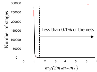
Figure 9: The distribution of m_3/(2m_1m_2-m_1^3) for the 90nm design testcase.
