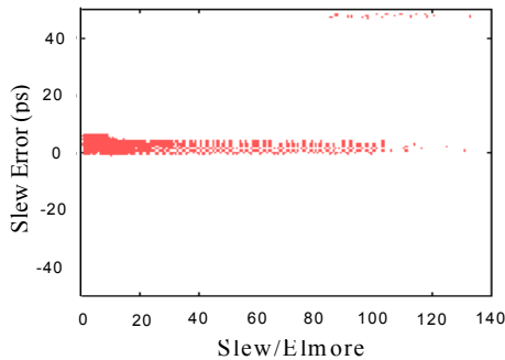
Figure 13: The calculated slew of the 90nm design testcase based on filtering algorithm with \phi=7 ps, \mu=7 , and \eta=2 .
