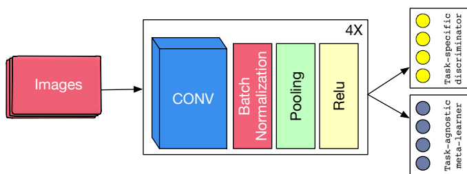
Figure 1: Meta-transfer learning model setup for miniImageNet dataset
