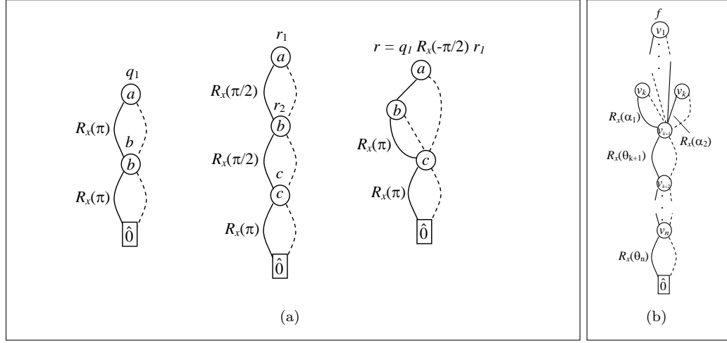
Fig. 6. (a) An example of performing apply operator on two RbDDs. In the first call of the apply operator, w_1 = [R_x(\pi)b]R_x(-\pi/2)[R_x(\pi/2)r_2] and w_0 = bR_x(-\pi/2)r_2 . The final figure is obtained after eliminating redundant nodes and edges. (b) A general RbDD structure with r -linear variables v_{k+1}, \dots, v_n .
