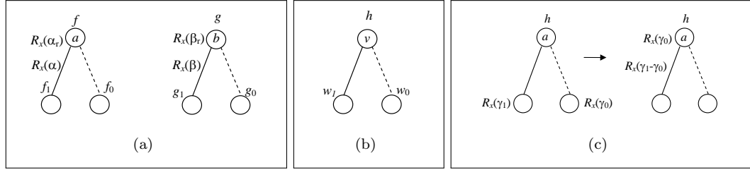
Fig. 5. (a) Operands for operation h = fR_x(\gamma)g . (b) The result of apply operator which adds a new node to the resulting RbDD h by using one of the three rules: if a < b (Rule 1), v = a , w_1 = [R_x(\alpha_r + \alpha)f_1]R_x(\gamma)g , w_0 = [R_x(\alpha_r)f_0]R_x(\gamma)g . If b < a (Rule 2), v = b , w_1 = fR_x(\gamma)[R_x(\beta_r + \beta)g_1] , w_0 = fR_x(\gamma)[R_x(\beta_r)g_0] . If a = b (Rule 3), v = a = b , w_1 = [R_x(\alpha_r + \alpha)f_1]R_x(\gamma)[R_x(\beta_r + \beta)g_1] , w_0 = [R_x(\alpha_r)f_0]R_x(\gamma)[R_x(\beta_r)g_0] . (c) Weight modification for the apply operator to maintain canonicity of the resulting RbDD.
