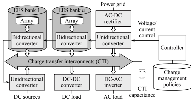
Fig. 1. The architecture of HEES systems.
