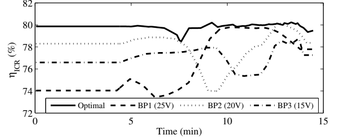
Fig. 10. Comparisons of the instantaneous charge replacement efficiency between the presented policy and baseline policies during the discharging process.
