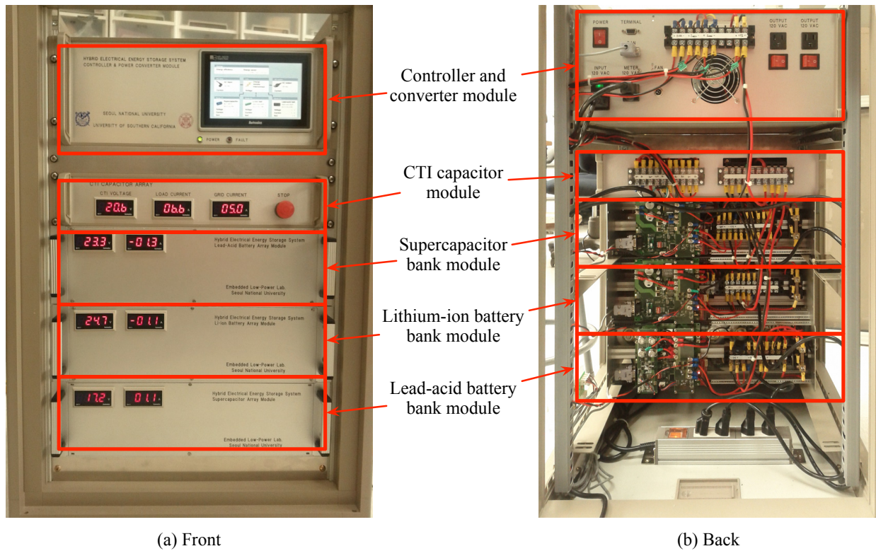
Fig. 2. The prototype of the proposed HEES system.
