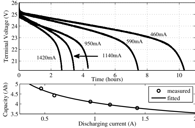
Fig. 8. Characterization of the lead-acid battery bank (top panel), and curve fitting of the rated capacities with respect to the discharging currents (bottom panel) to find the Peukert constant.
