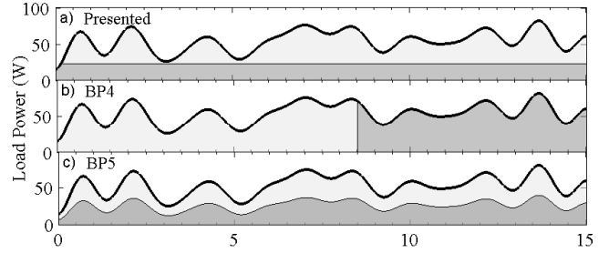
Fig. 11. Power assignments by the presented GCR policy (a), BP4 (b), BP5 (c) for the 15-min load profiles in Table V. Light and dark gray areas denote amounts of energy drawn from the supercapacitor bank and the lead-acid battery bank, respectively.
