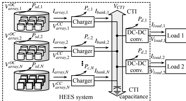
Fig. 3. Block diagram of HEES systems for a charge replacement problem.
