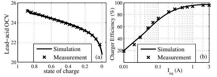
Fig. 5. Comparison of the circuit model simulation results with the measured battery terminal voltage of the lead-acid battery bank in the HEES prototype (a) and the conversion efficiency of a LTM4607 power converter (b).
