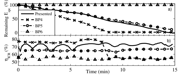
Fig. 12. Comparisons of the normalized remaining energy in the supercapacitor bank (a) and the instantaneous charge replacement efficiencies (b) obtained by the presented GCR policy and baseline policies, for the 15-min load profiles in Table V.
